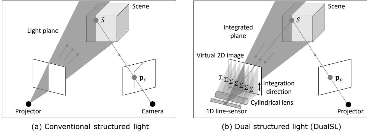
Figure 3.1: DualSL compared with traditional SL. Depth from SL can be obtained by performing ray-plane triangulation. For traditional SL, the ray is from camera pixel, and plane is formed by center of projection and a column of the projector. In DualSL, ray is from projector pixel, and plane is formed by a line sensor pixel with cylindrical optics.
