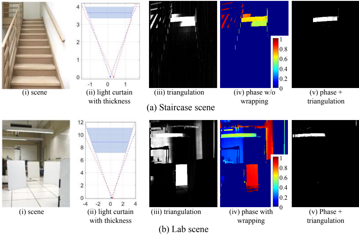
Figure 4.9: Using line CW-TOF sensor. For both scenes, we show that fusing (iii) triangulation with (iv) phase information leads to (v) thinner light curtains without any phase wrapping ambiguity.
